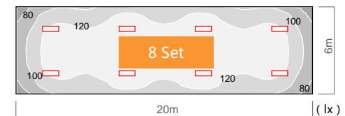
Isolux diagram Face
